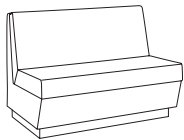
straight unit d 27.5" w 48", 60" or 72" h 35"
